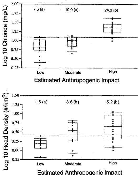
FIGURE 2.—Relationships between the qualitative grouping of anthropogenic impact for 60 Florida lakes and both the chloride concentrations and road densities measured for those lakes. Average chloride concentrations and road densities for each anthropogenic impact group are recorded above the box plots, and averages with different letters are significantly different ( P < 0.05 ), as determined by one-way analysis of variance, followed by a Tukey–Kramer HSD test. The long horizontal line represents the grand mean of all values. The quantile box plots show the median as a line across the middle of the box, the 25th and 75th quantiles are the ends of the box, and the 10th and 90th quantiles are the short horizontal lines below and above the box.
